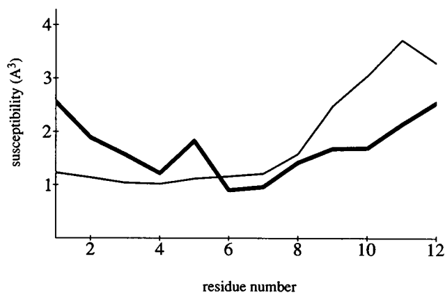
FIGURE 2 Susceptibility \alpha ( \text{Å}^3 ) of deca-alanine as a function of residue number. Molecular dynamics ( bold ); normal modes ( light ).
