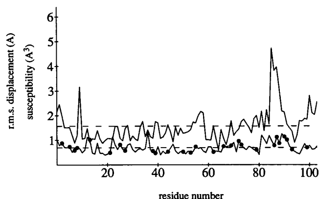
FIGURE 10 R.m.s. fluctuations ( \text{Å} ) of each residue (lower curve), and susceptibility \alpha ( \text{Å}^3 ) at the \alpha -carbon (upper curve), as a function of the residue number. (Residue zero represents the methyl carbon blocking the N -terminus.) The two dashed lines indicate the average values for the two curves. Dots superimposed on the lower curve signal the location of charged residues along the polypeptide chain.
