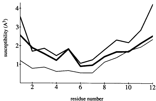
FIGURE 4 Susceptibilities ( \text{Å}^3 ) of deca-alanine, for different trajectory lengths, as a function of residue number. 60 ps ( bold ), 30 ps ( medium ), and 15 ps ( light ).
