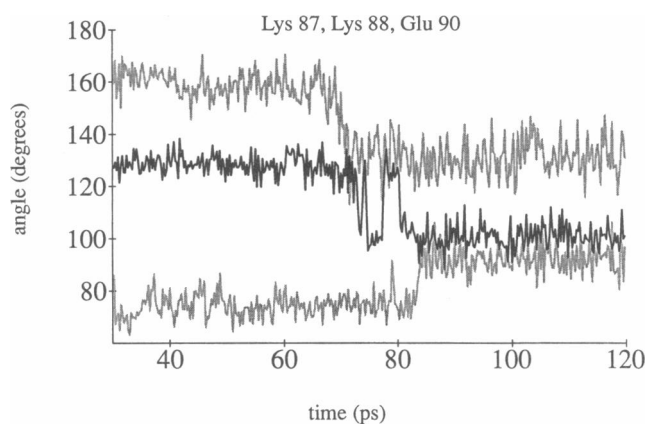
FIGURE 16 The angle N-C_{\alpha}-N_i plotted as a function of time for lysines 87 (light, lower) and 88 (light, upper); the angle N-C_{\alpha}-C_i as a function of time for Glu 90 (bold).
